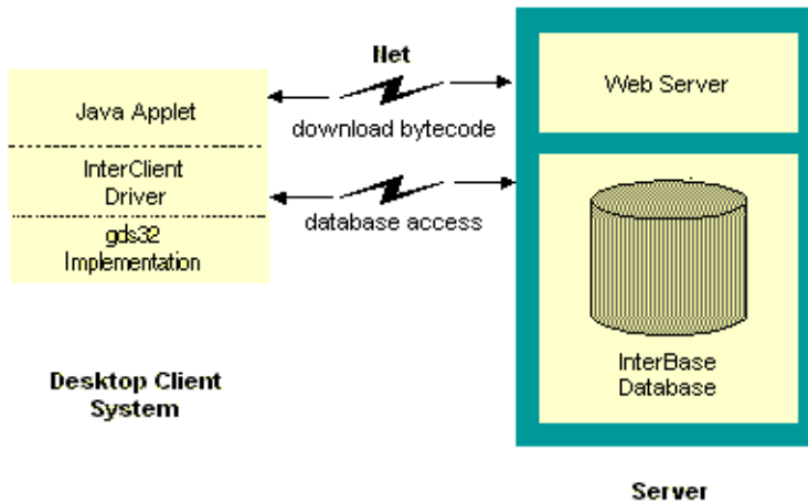
Figure 4.2 InterClient architecture
