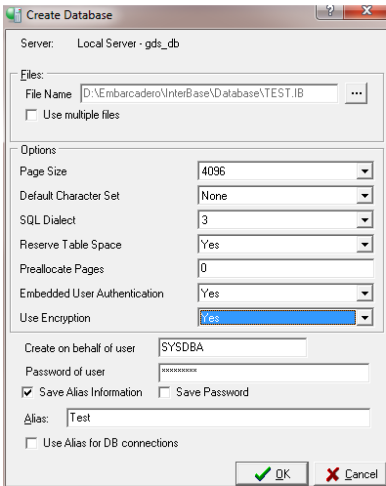
Figure 14.1 Enabling EUA and encryption
