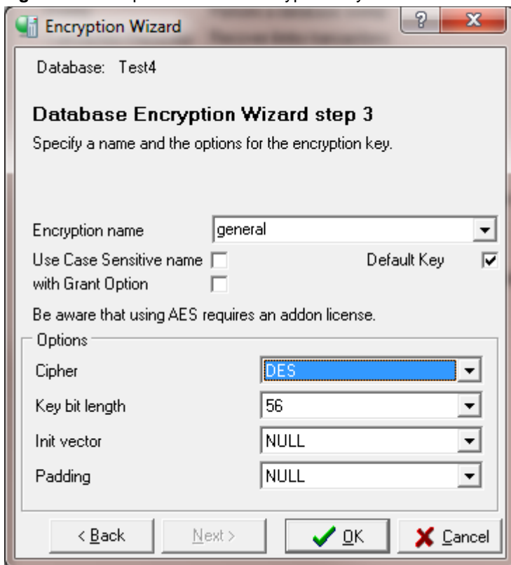
Figure 14.5 Step 3: Create an encryption key
