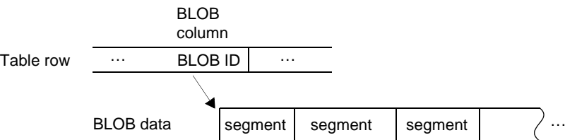
Figure 4.1 Blob relationships
