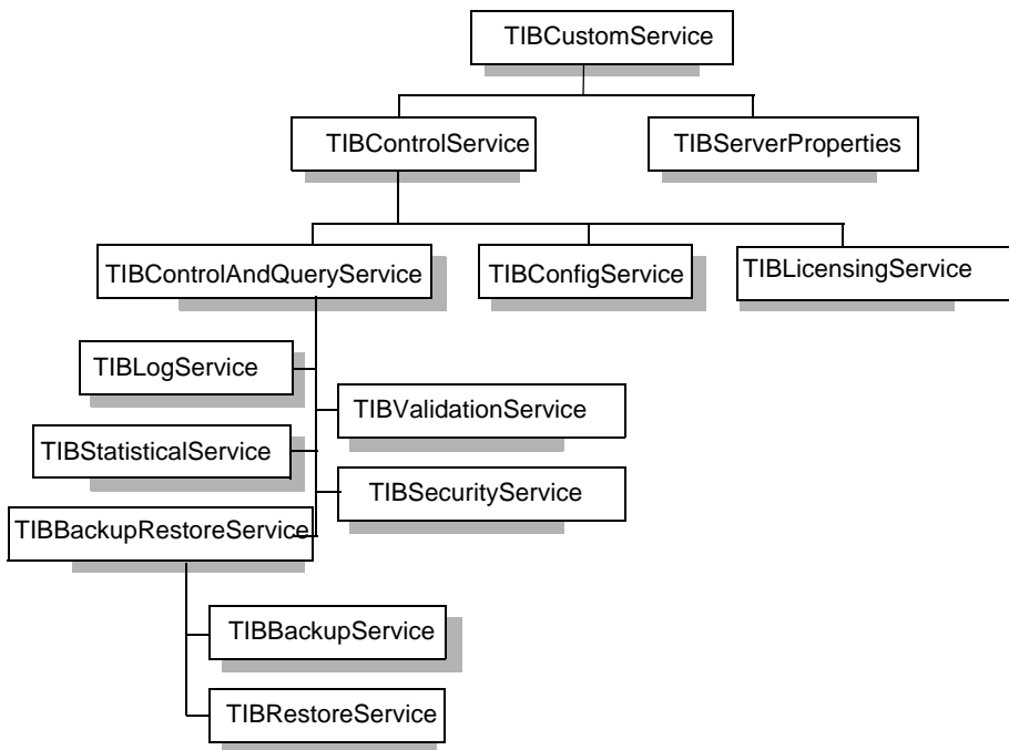
Figure 12.1 InterBase service component hierarchy
